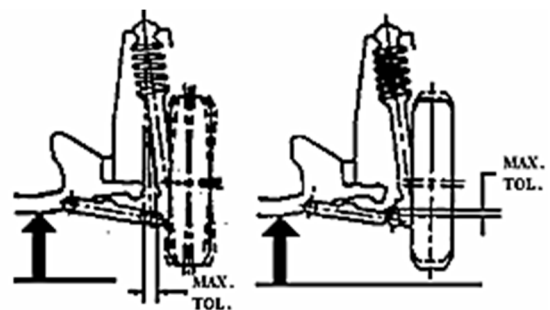
MACPHERSON STRUT
