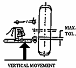
SPRING OR TORSION BAR ON LOWER CONTROL ARM
