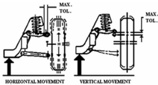
SPRING ON UPPER CONTROL ARM
