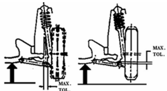
MACPHERSON STRUT
